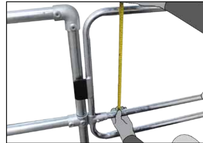
Q. Use a measuring tape to ensure gap between top rail and mid rail is no more than 470mm. Adjust if necessary.
